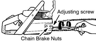
Adjusting Screw - 1/4 Turn
